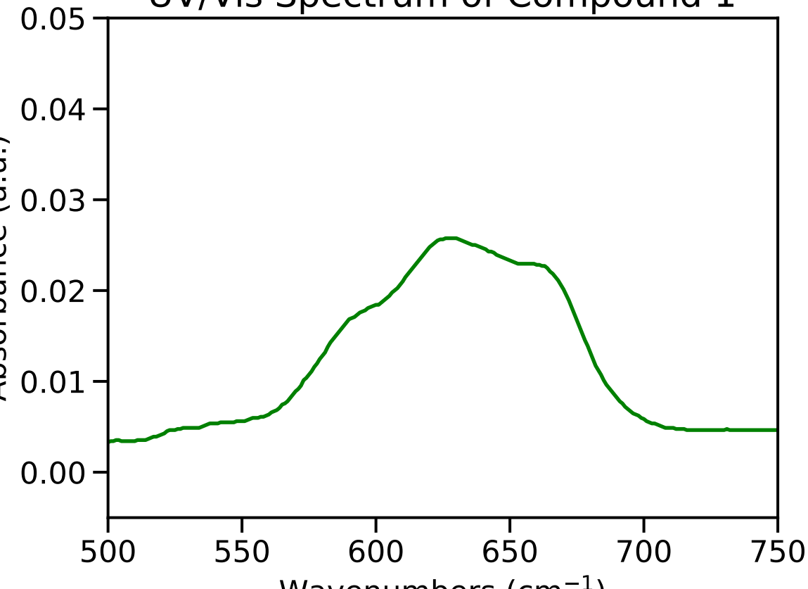
UV/Vis Spectrum of Compound 1
